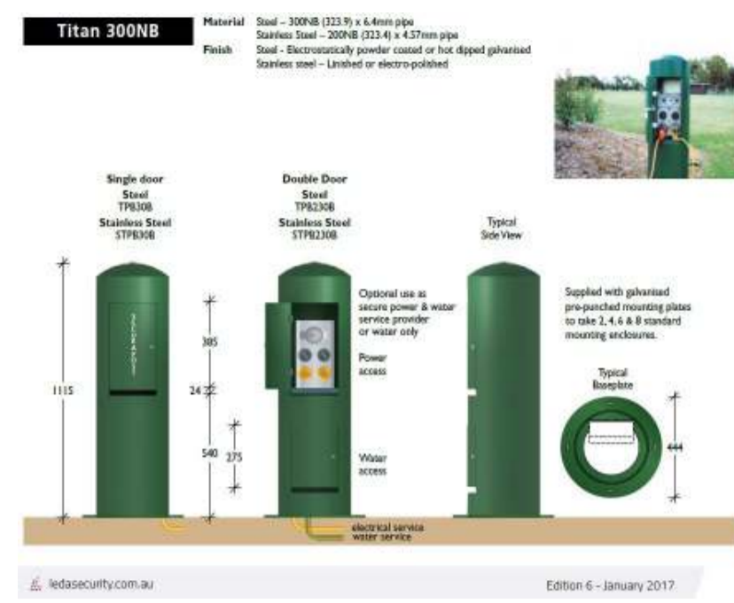
Titan 300 Power Distribution Bollard From Leda
