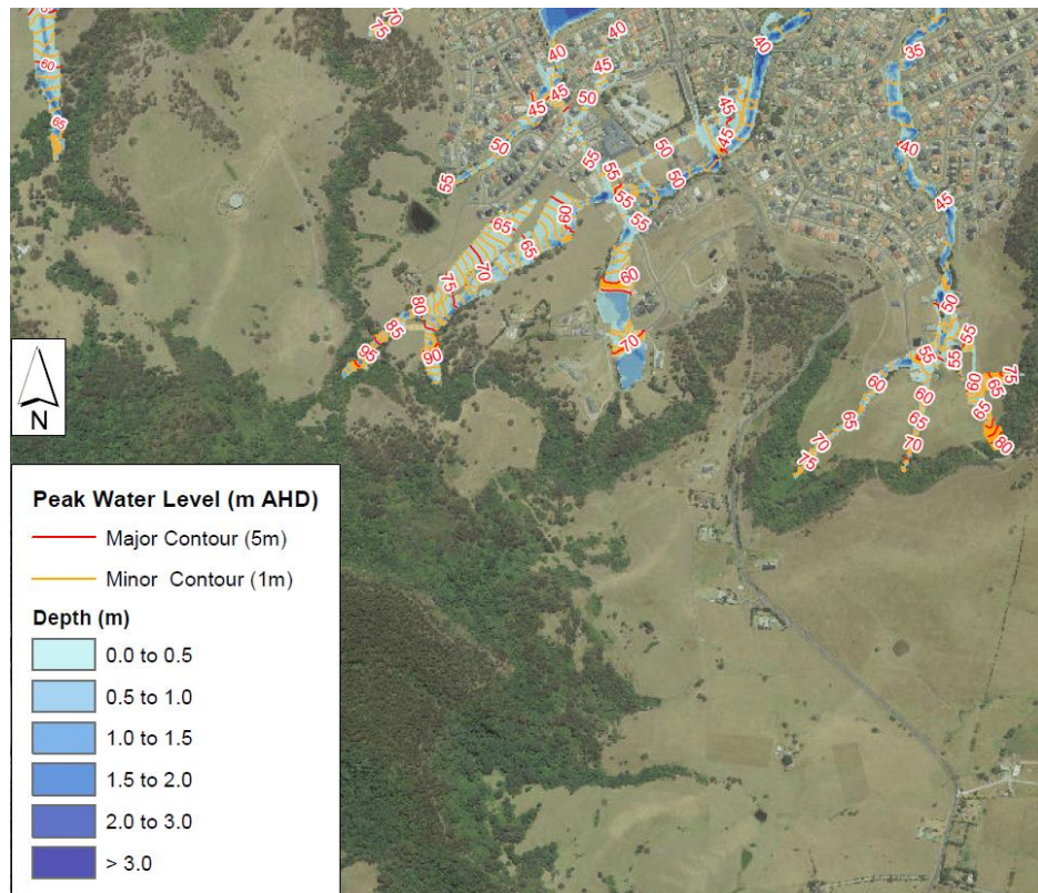
Figure 14 Flood Depths and Flood Level Contours (WMAwater 2017)
