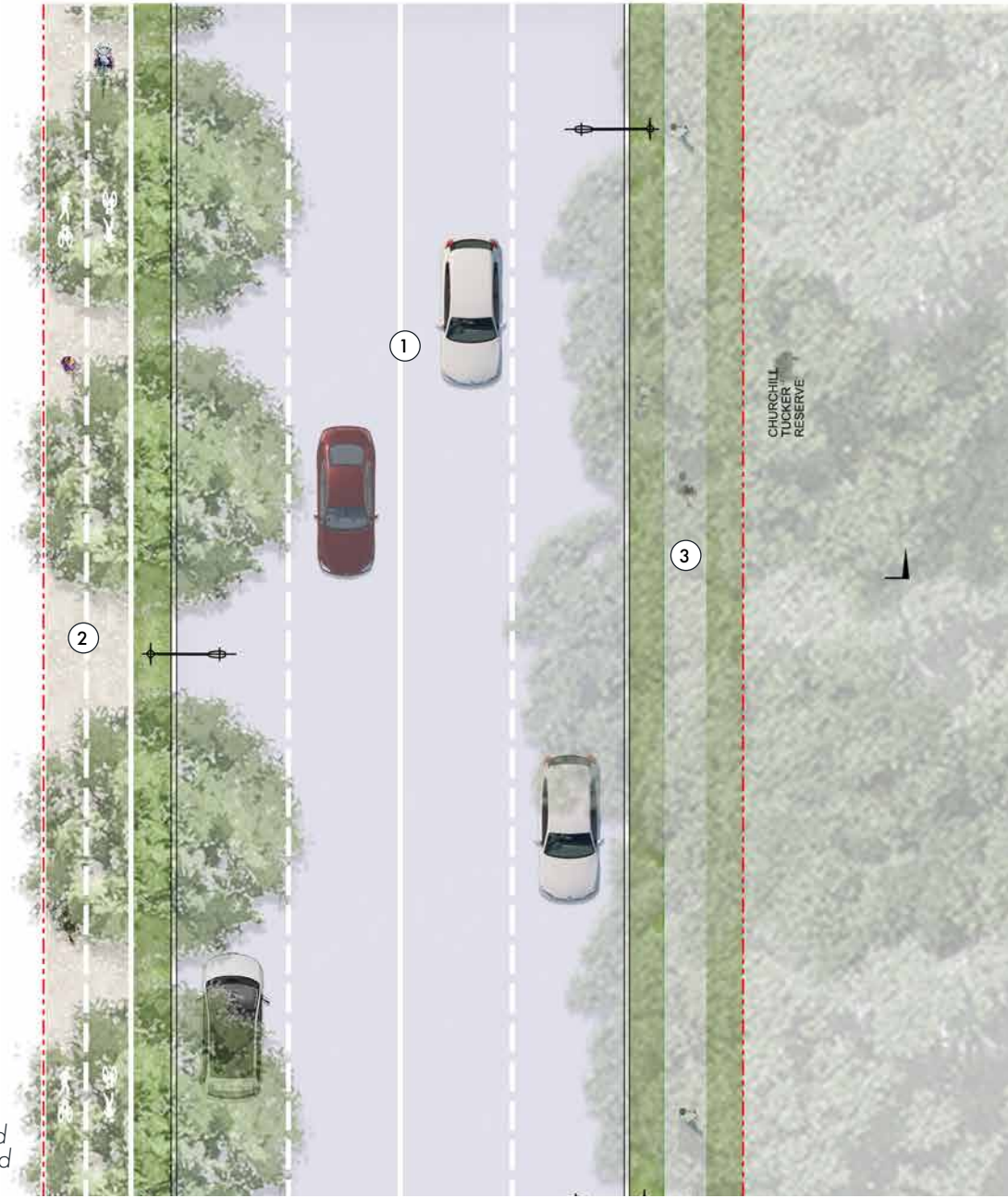
Figure 64. Mary Street East - Typical Plan
