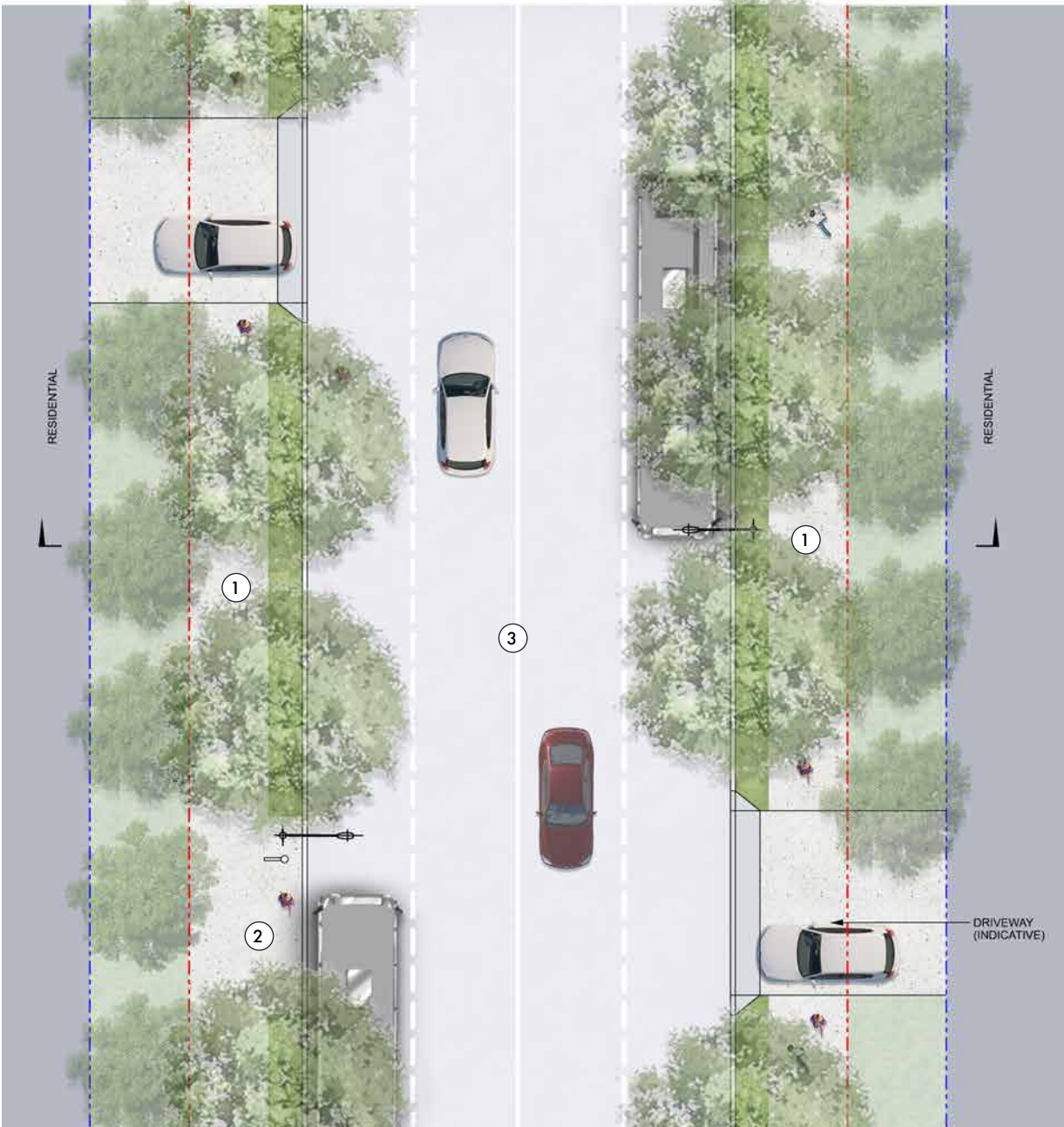
Figure 58. Averill Street - Typical Plan
