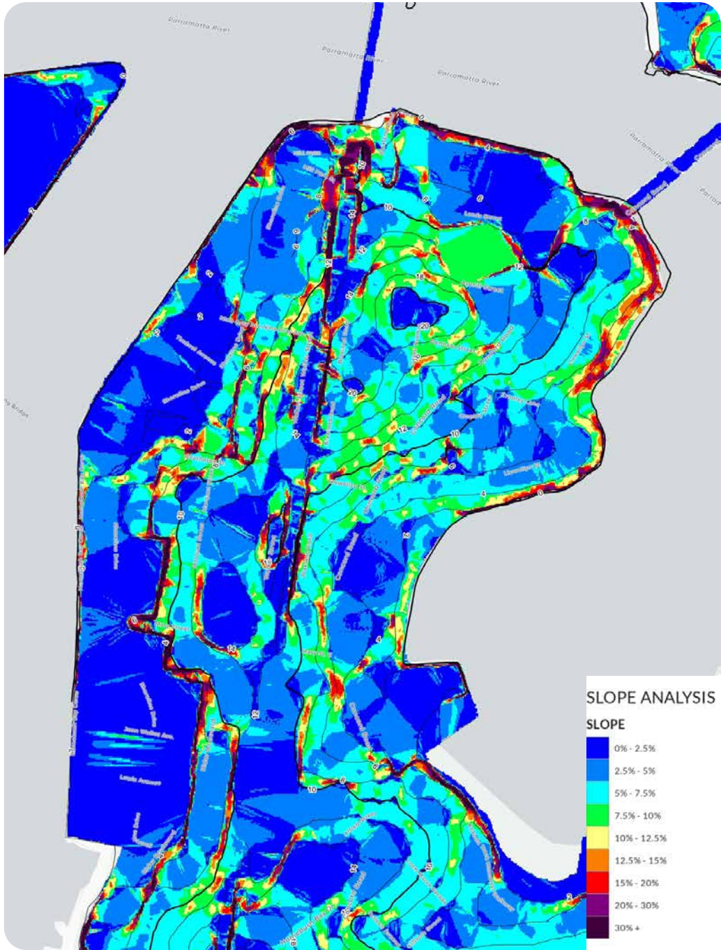
Figure 9. Existing Slope Map
