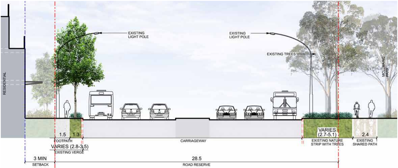
Figure 35. Concord Road South (Mcllwaine Park) - Typical Section
