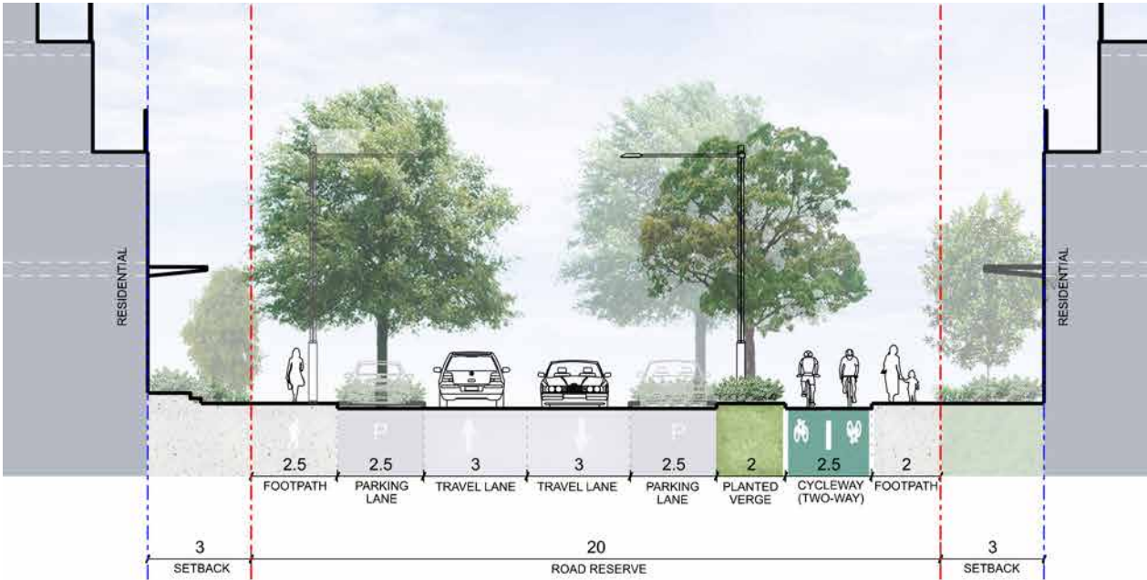
Figure 59. Denham Street, Denham Street Extension (New Street) and Llewellyn Street - Typical Section
