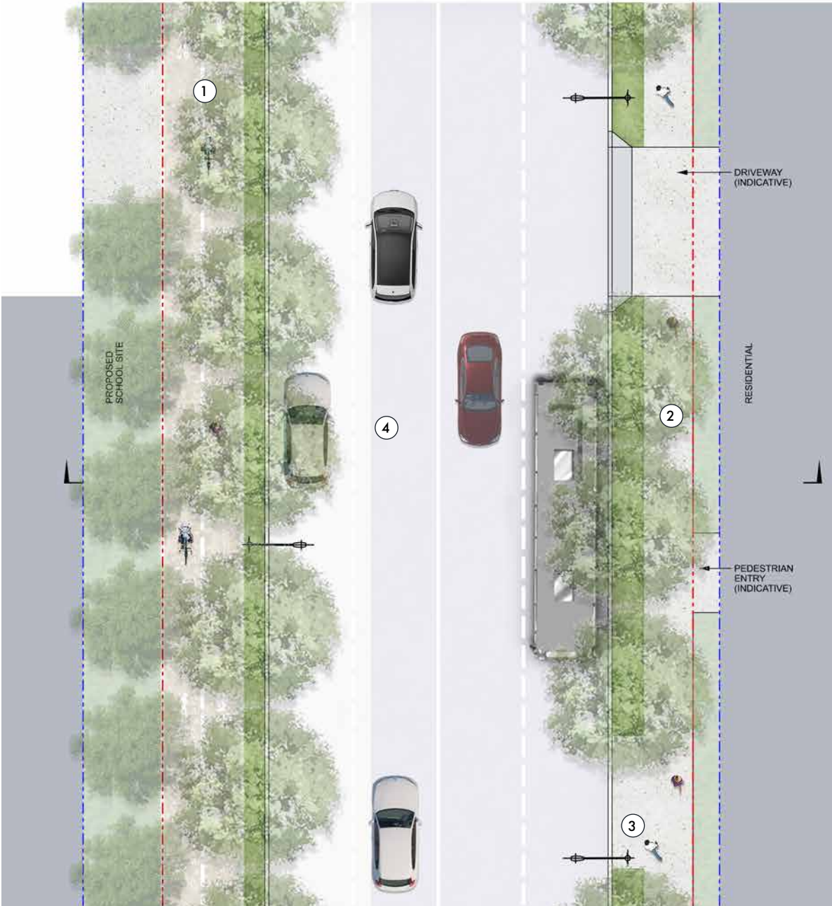
Figure 50. Cavell Avenue North - Typical Plan
