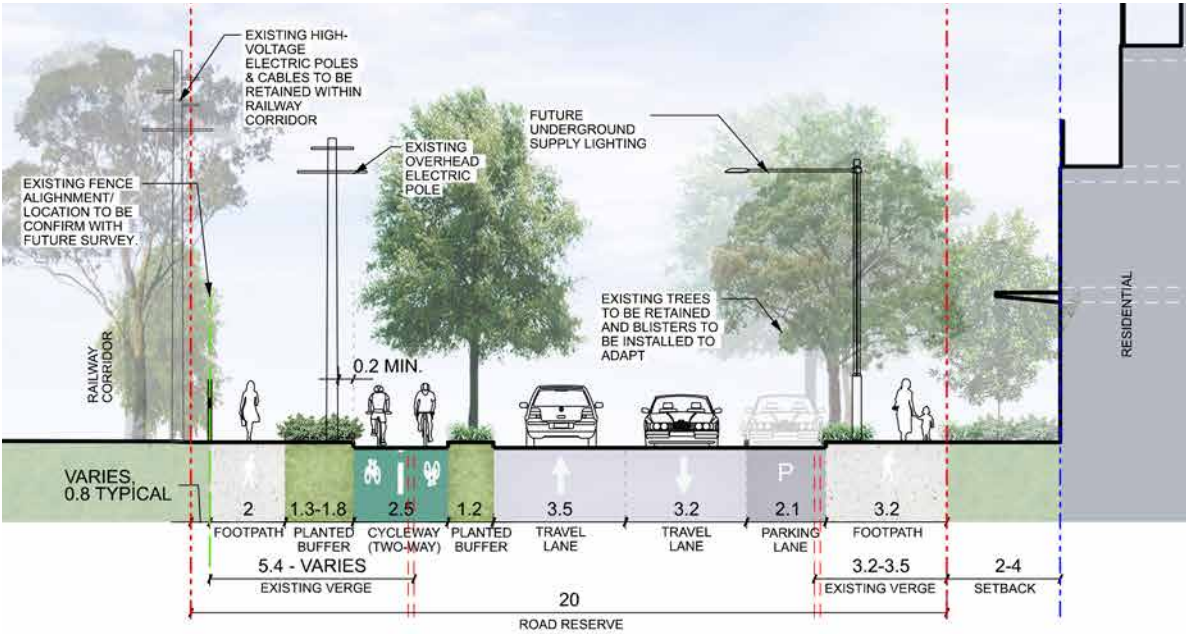
Figure 37. Blaxland Road North - Typical Section
