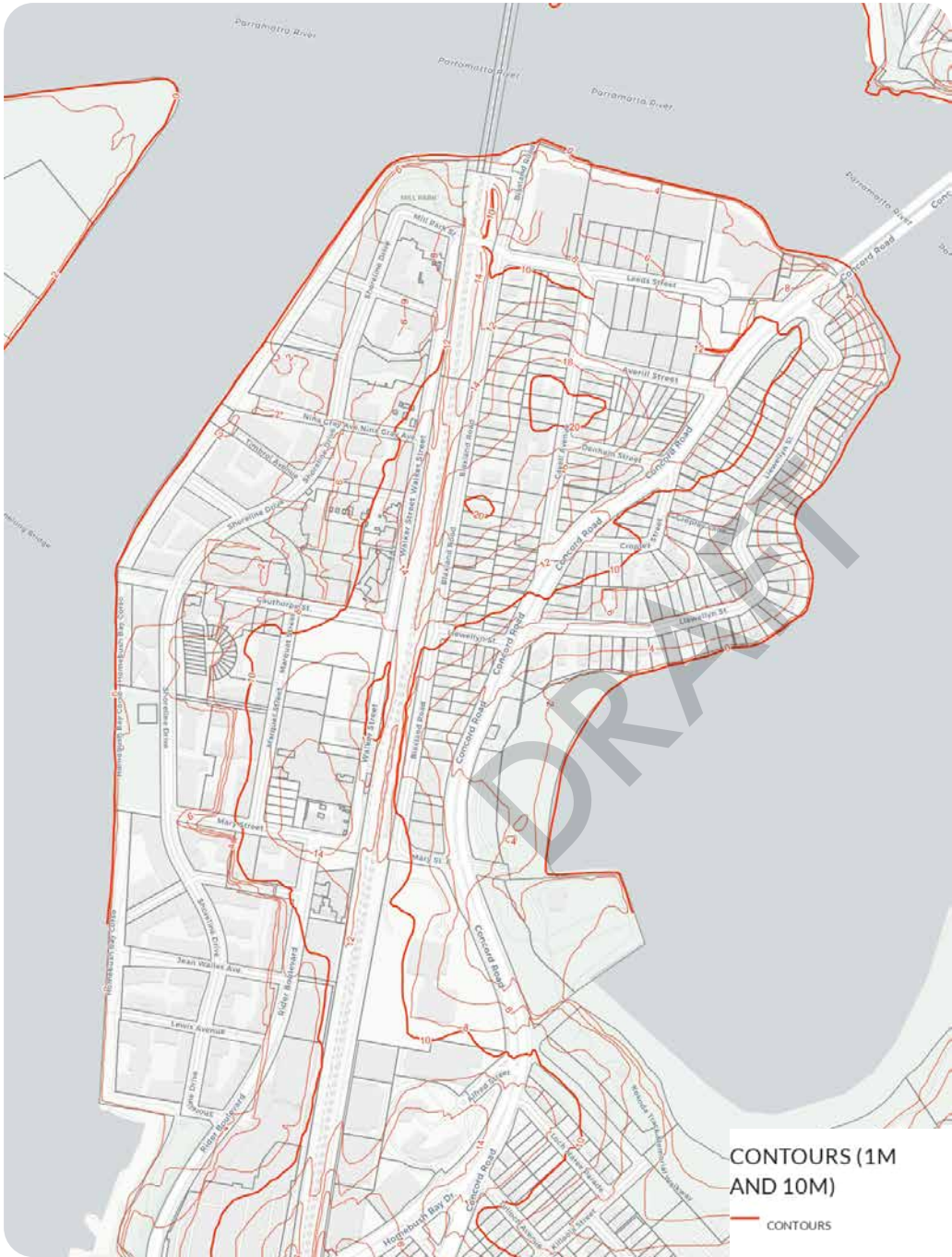
Figure 8. Existing Elevation Map
