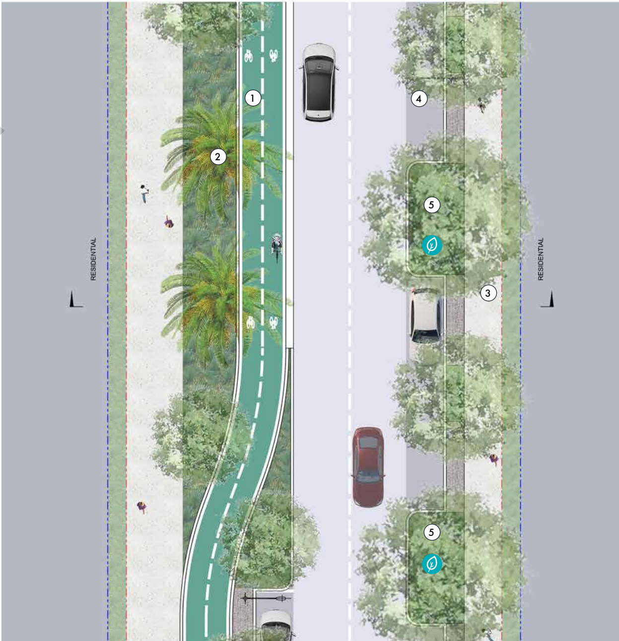
Figure 56. Cavell Avenue South - Scenario 2 Plan
