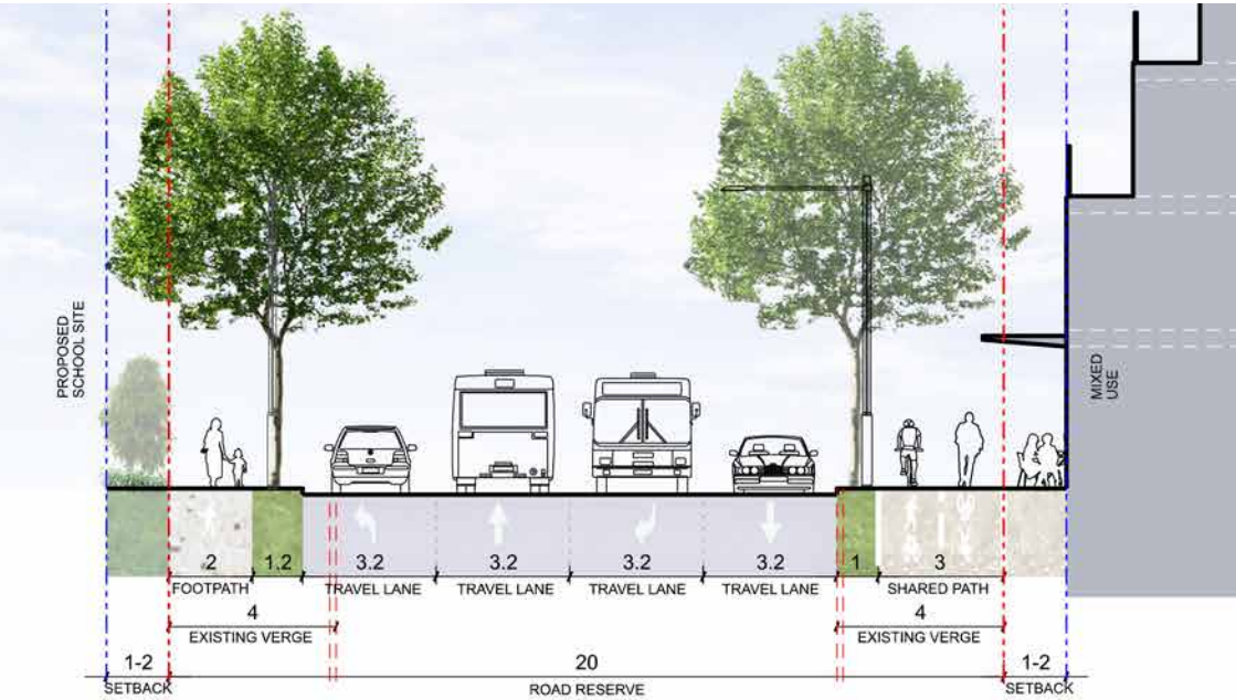
Figure 45. Leeds Street West - Typical Section
