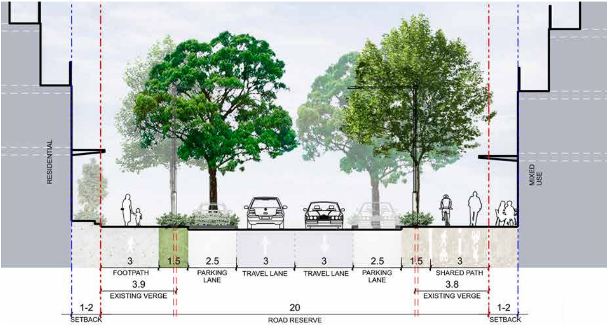
Figure 47. Leeds Street East - Typical Section
