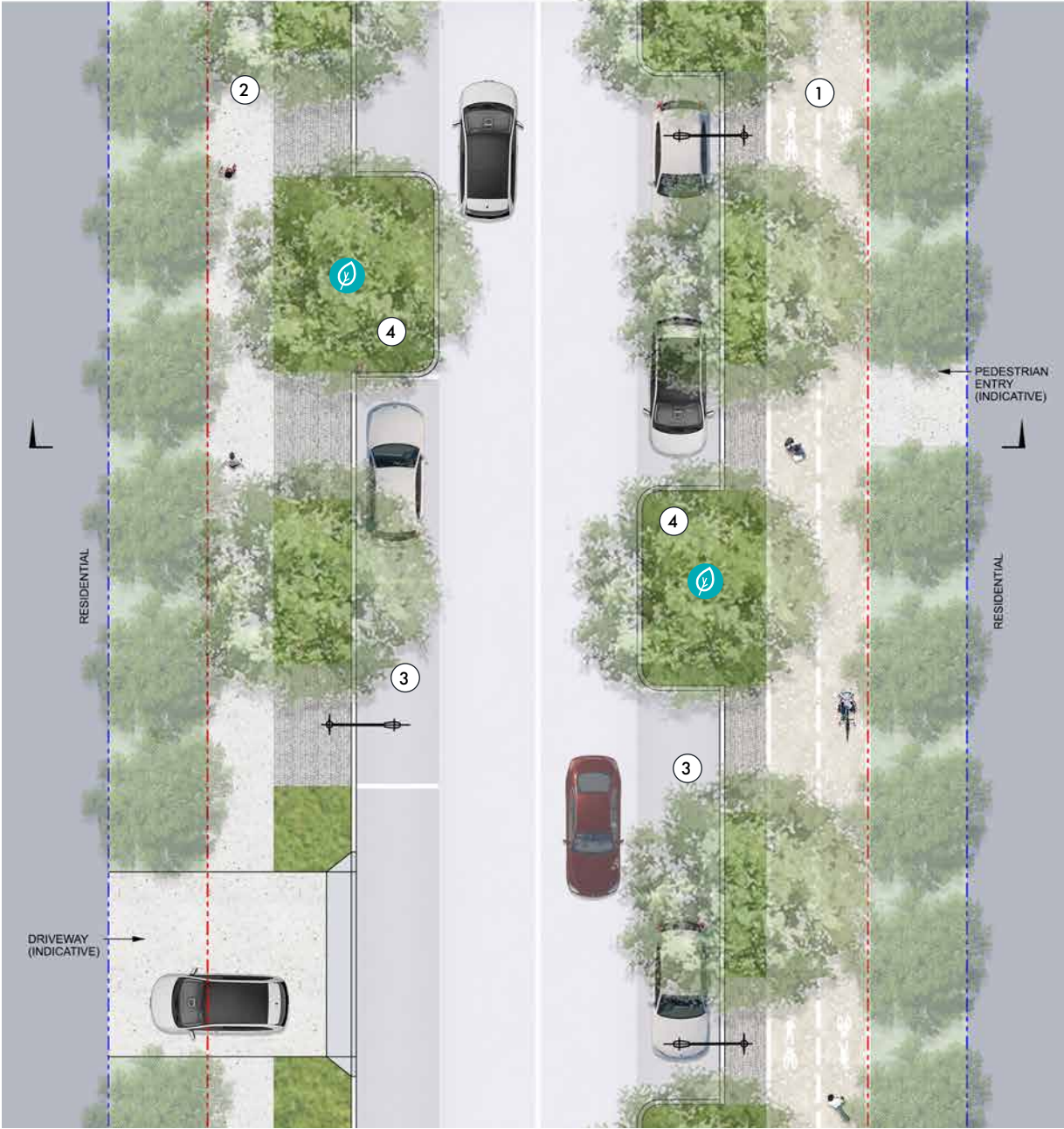
Figure 62. New Street with Shared Path - Typical Plan
