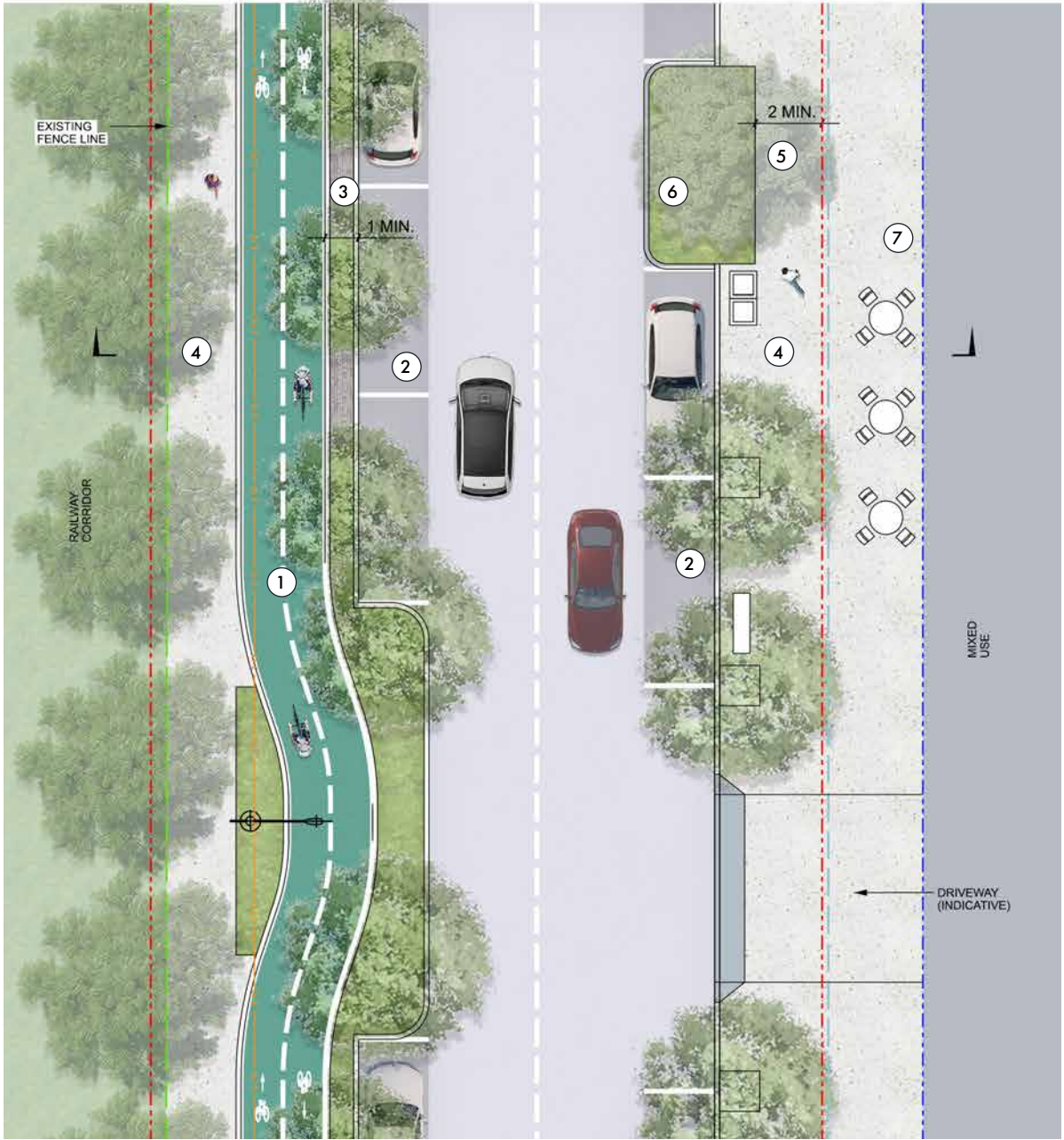
Figure 42. Blaxland Road South (Between Llewellyn Street and Train Station) - Plan
