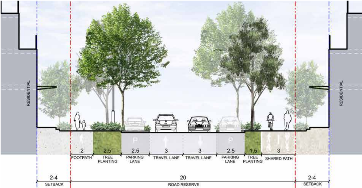
Figure 61. New Street with Shared Path - Typical Section
