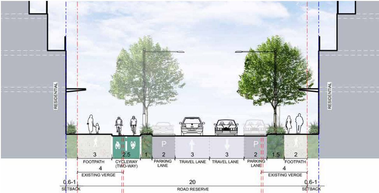
Figure 51. Cavell Avenue South - Typical Section
