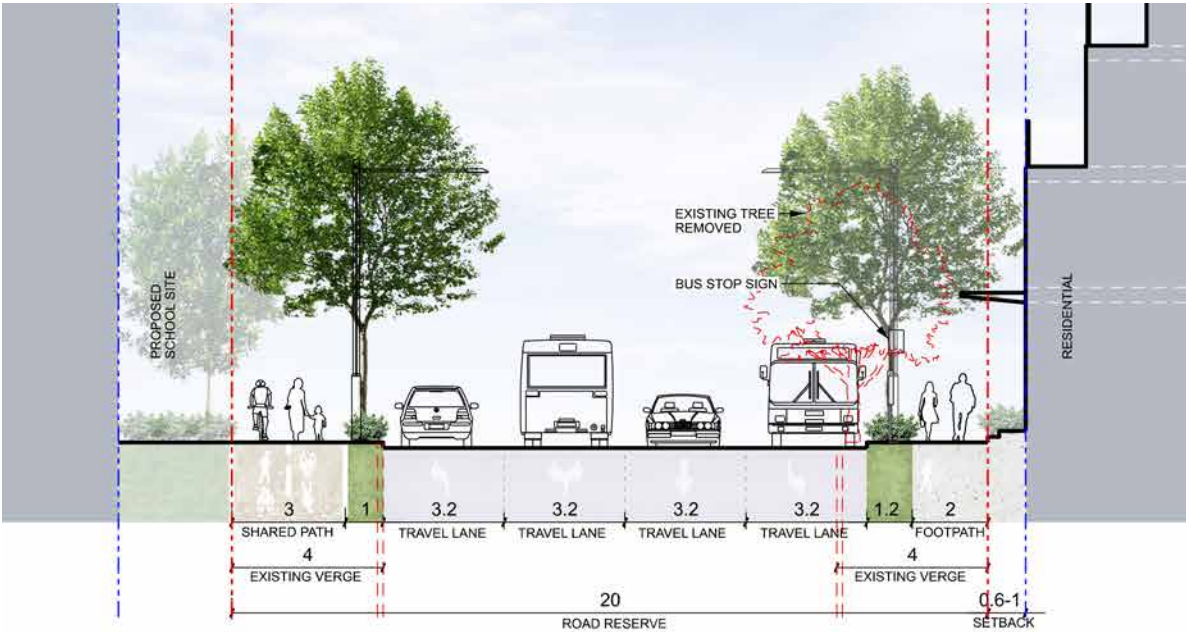
Figure 49. Cavell Avenue North - Typical Section
