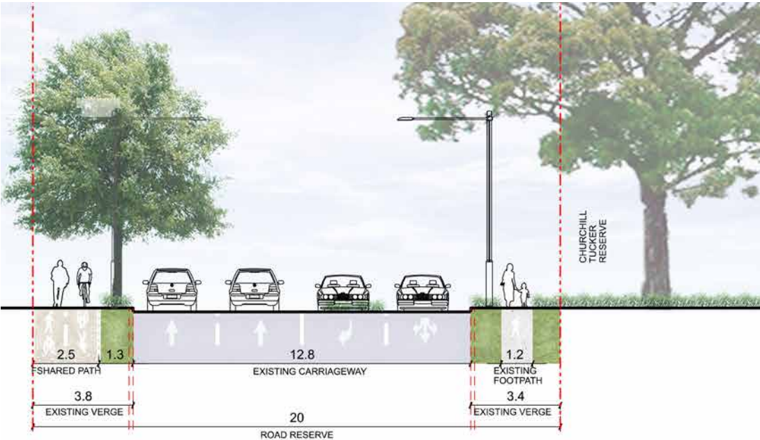
Figure 63. Mary Street East - Typical Section
