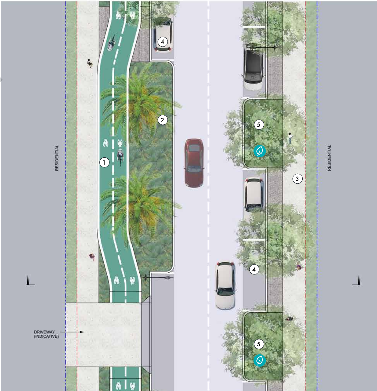
Figure 54. Cavell Avenue South - Scenario 1 Plan
