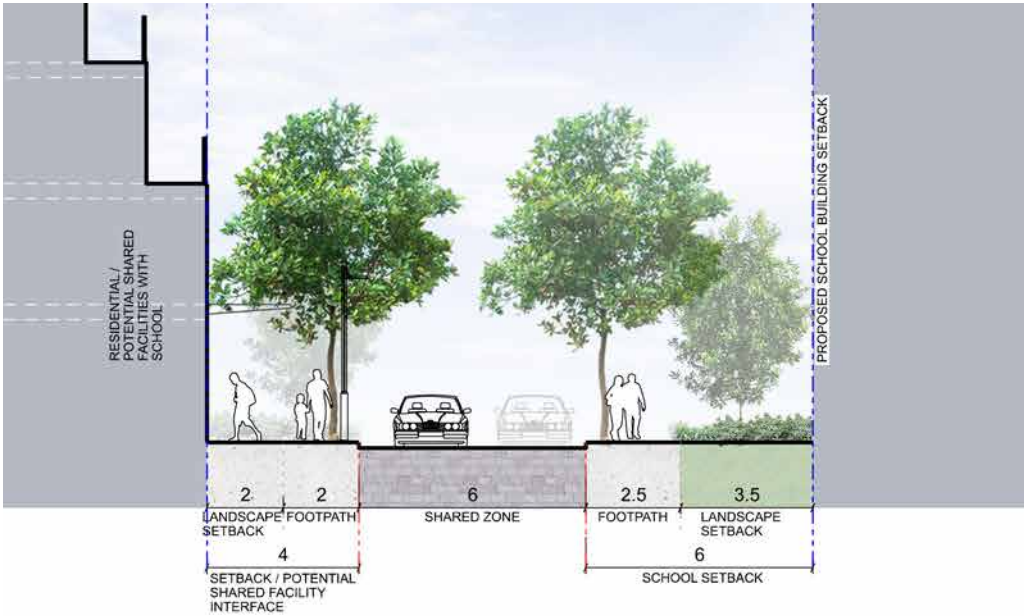
Figure 65. Shared Zone - Typical Section
