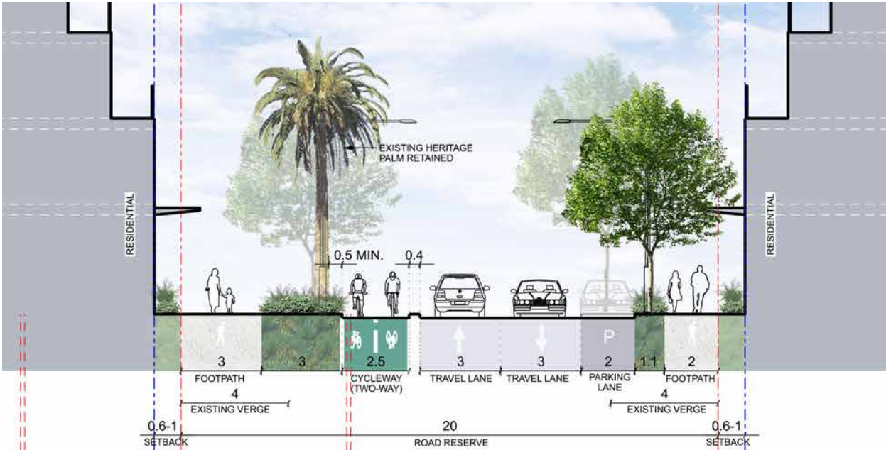
Figure 55. Cavell Avenue South - Scenario 2 Section
