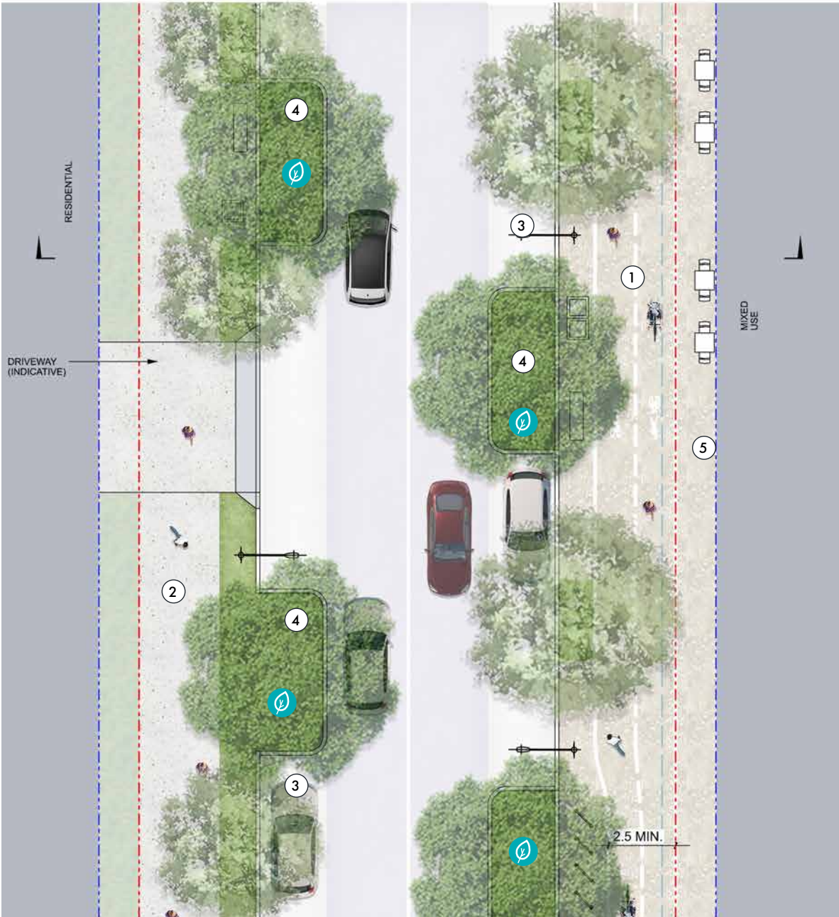
Figure 48. Leeds Street East - Typical Plan
