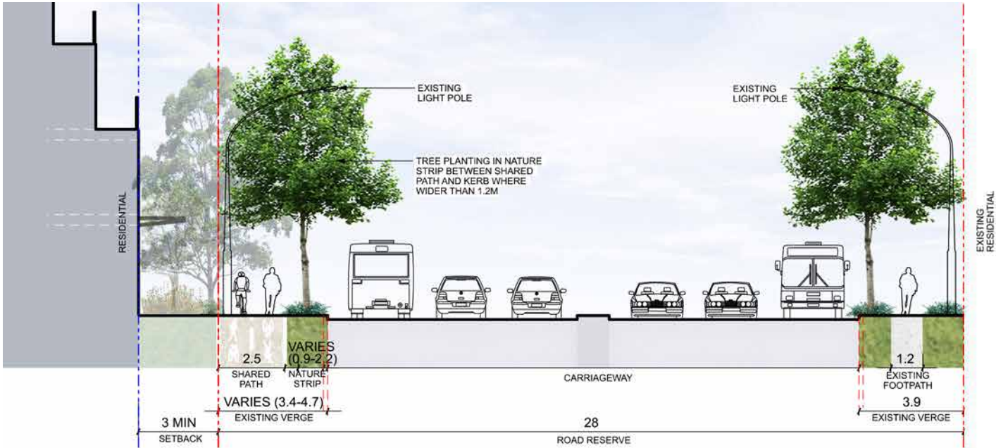
Figure 33. Concord Road North - Typical Section
