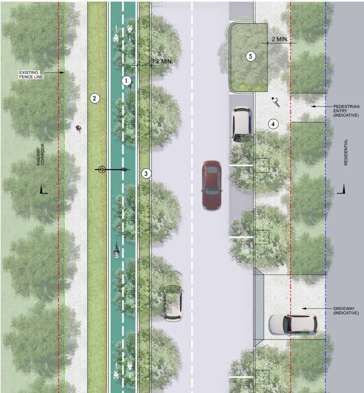
Figure 38. Blaxland Road North - Typical Plan
