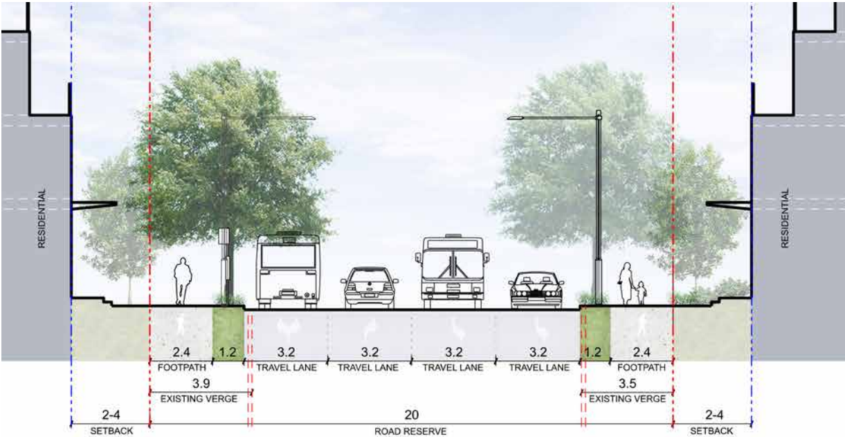
Figure 57. Averill Street - Typical Section
