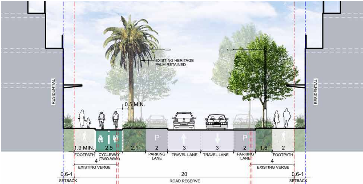
Figure 53. Cavell Avenue South - Scenario 1 Section
