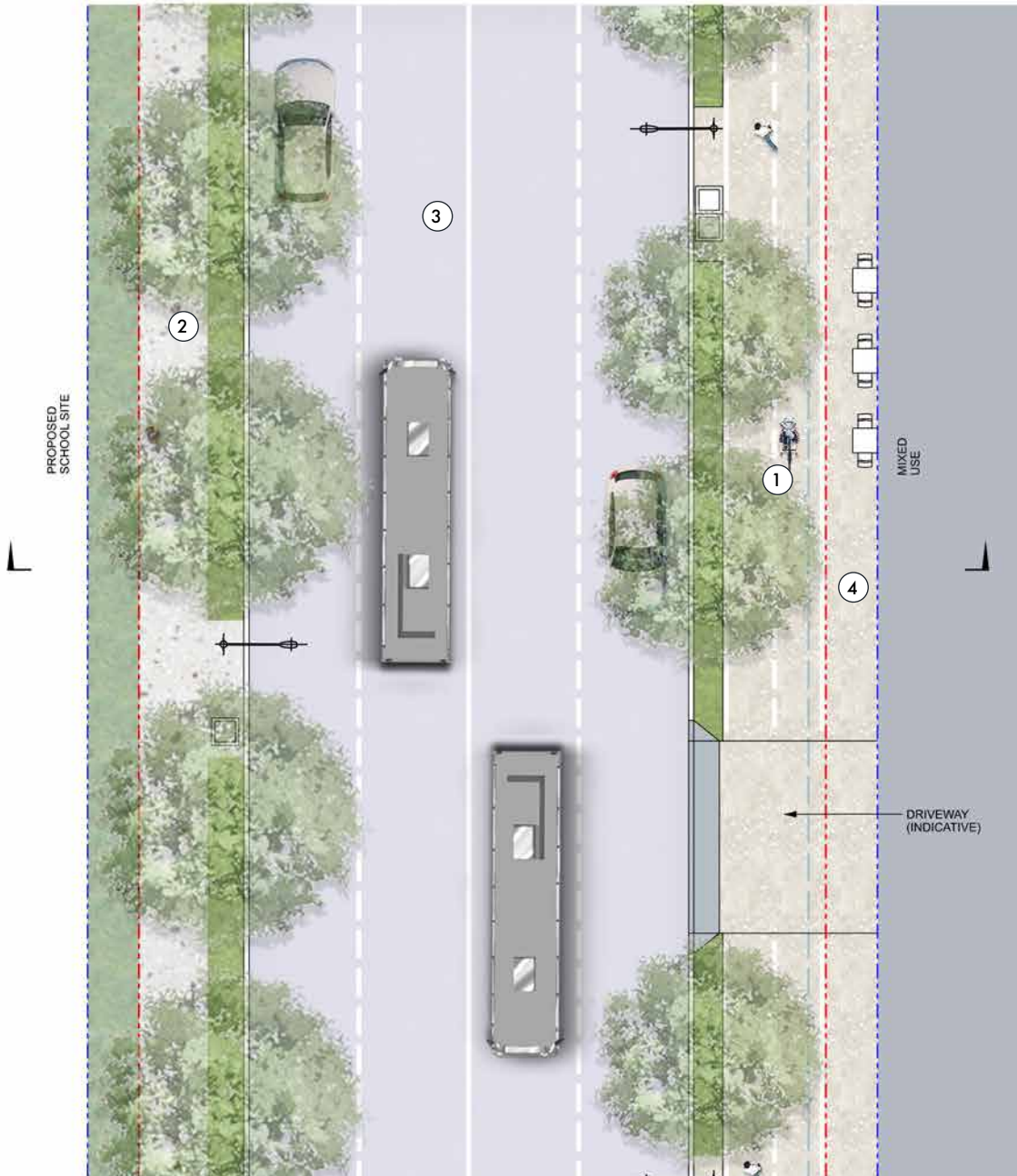
Figure 46. Leeds Street West - Typical Plan
