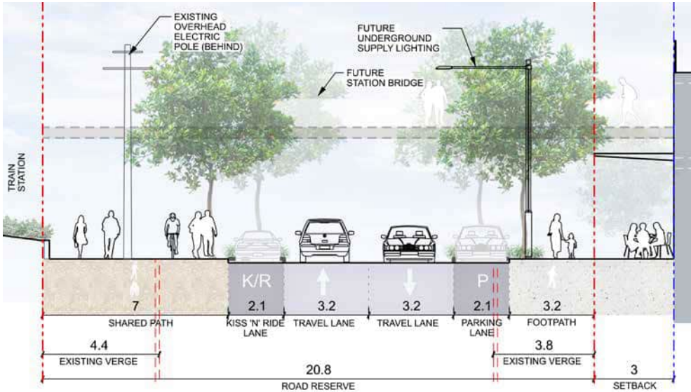
Figure 43. Blaxland Road South Station Frontage - Section
